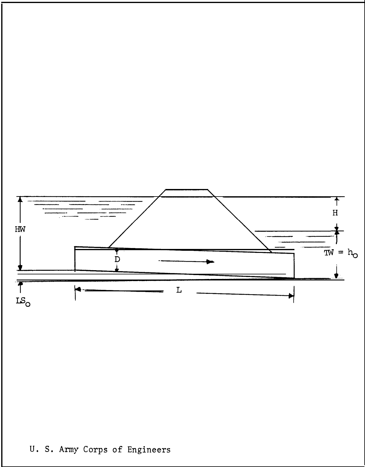
Figure B-18, Tailgate elevation at or above top of culved.
